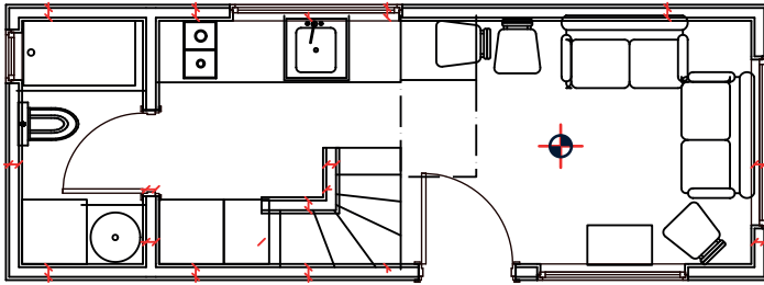
Zemin Kat / Ground floor
