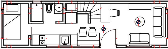
Zemin Kat / Ground floor
